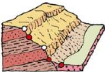
崖錐斜面と崖壁
